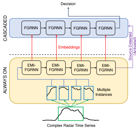
Figure 2: MSC-RNN architecture – the lower EMI-FastGRNN runs continuously, while the upper FastGRNN is invoked only for legitimate displacements
